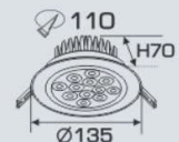
AFC 512 LED 12W 646.000
