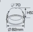
AFC 586 LED 7W 345.000
